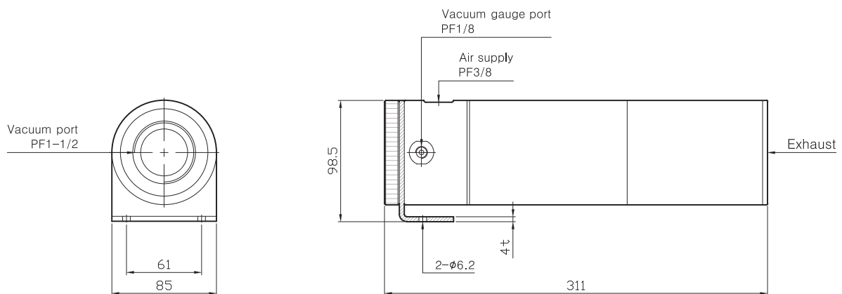
SMR1085/1285
