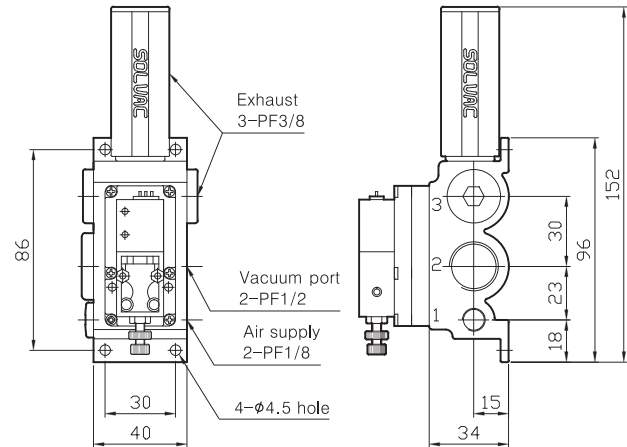
VSM/VSX 'D' type (with switch) VSM/VSX(02D, 04D, 06D)
