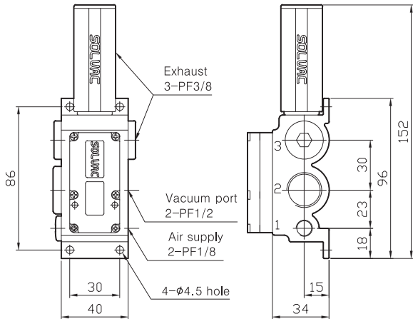
VSM/VSX 'D' type (without switch) VSM/VSX(02D, 04D, 06D)
