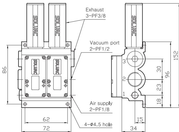
VSM/VSX 'D' type (without switch) VSM/VSX(08D, 10D, 12D)
