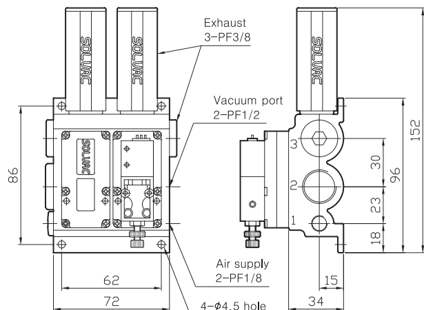
VSM/VSX 'D' type (with switch) VSM/VSX(08D, 10D, 12D)
